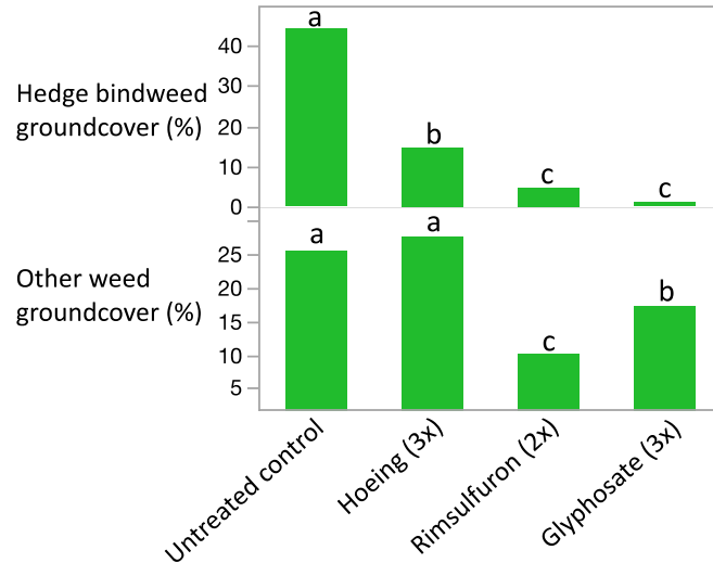
Figure 1. Carryover effects on hedge bindweed and other weeds as represented by percent groundcover on June 5, 2019, nearly one year after the treatments were implemented. The effect of treatments on weed density was similar to weed groundcover (data not shown). For each graph, bars with the same letter are not significantly different (Fisher's Protected LSD, P \leq 0.05 ).
